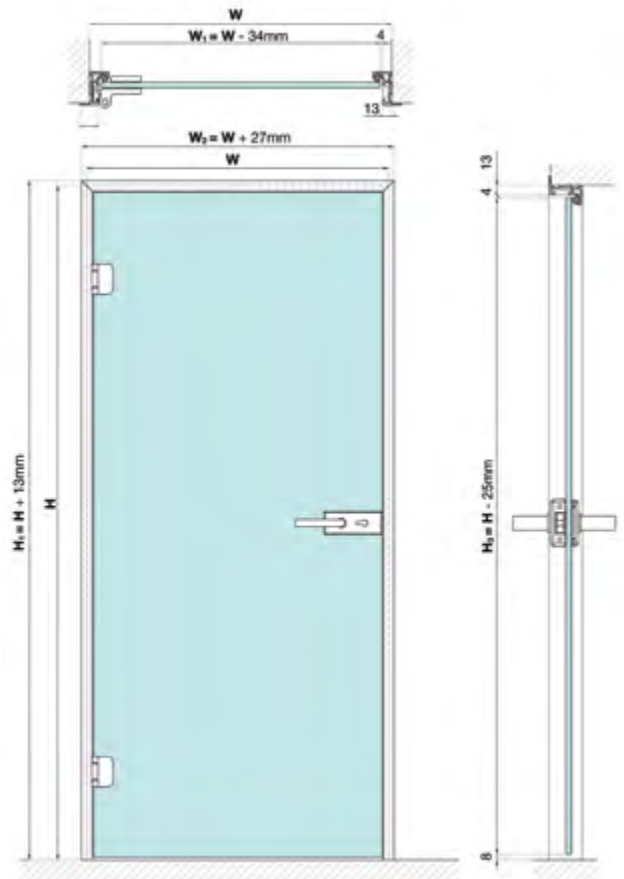
Z-Type Door Frame
