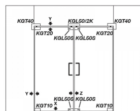
Installation Dimensions X: 7-10mm Y: 2-4mm Z: 3-5mm
