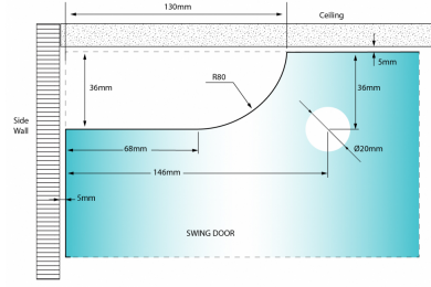
Top Patch Cut Out - KGT2055-PLUS
