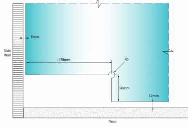
Bottom Patch Cut Out - KGT1055-AUTG100
